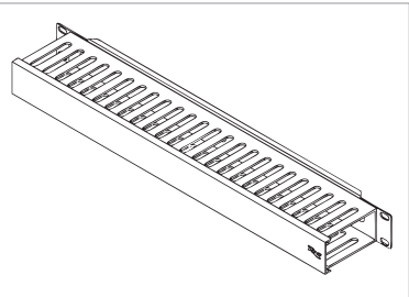
Single Horizontal Finger Ducts ICCMSMA41 1.58" H x 3.15" D, 1 RMS ICCMSMA42 3.15" H x 3.15" D, 2 RMS
