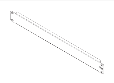
Blank Panels ICCMSCMPB1 1.75"H x 19"W, 1 RMS ICCMSCMPB2 3.50"H x 19"W, 2 RMS ICCMSCMPB3 5.25"H x 19"W, 3 RMS
